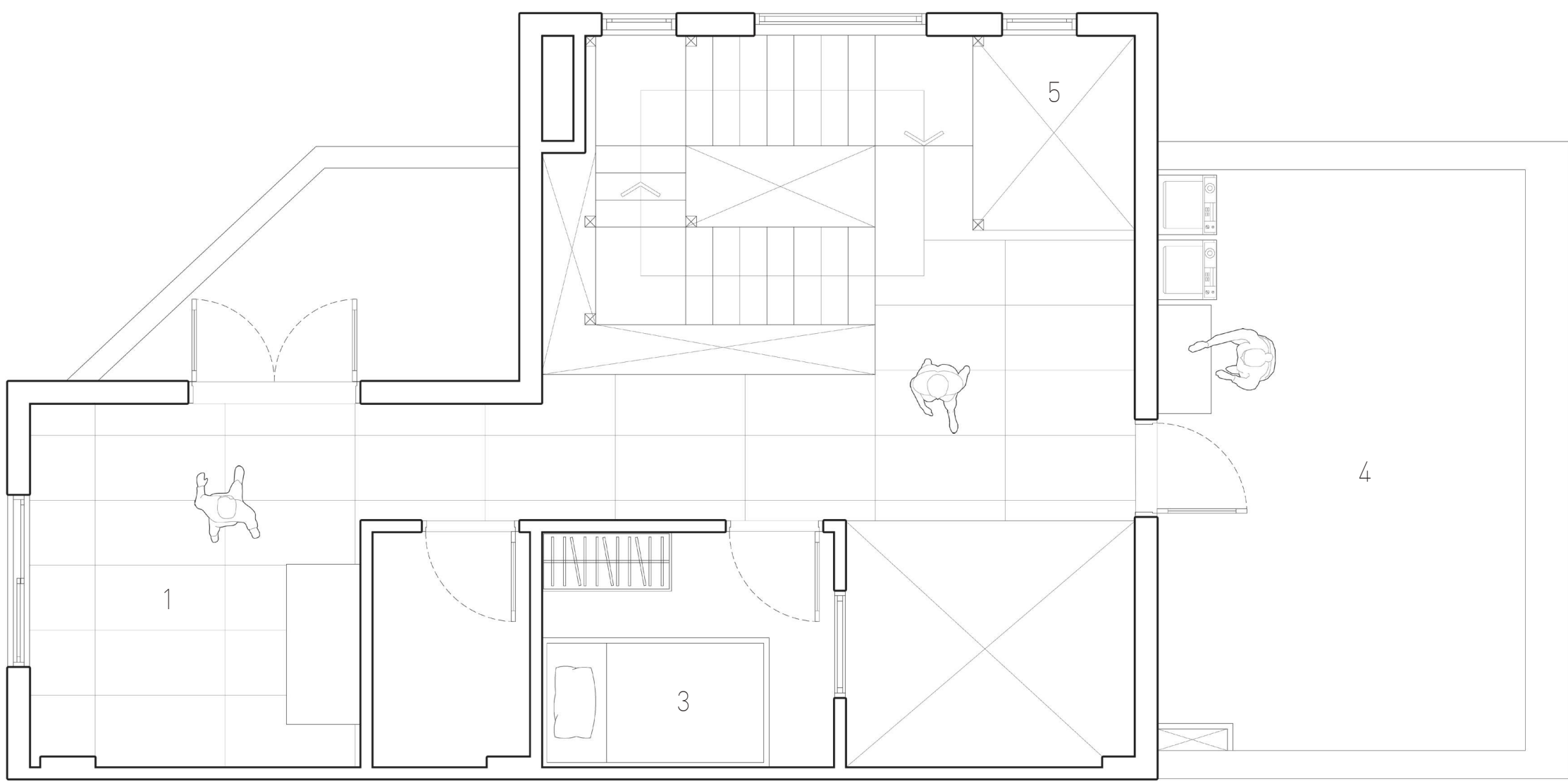
MẶT BẰNG TẦNG BỐN | 4TH FLOOR PLAN
